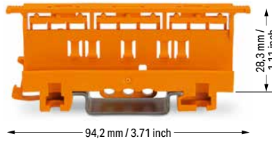
Mounting carrier; for 2-, 3- and 5-wire splicing connectors (6 mm 2 ); 19.3 mm wide
