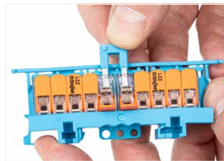
Remove the jumper from open clamping units.
